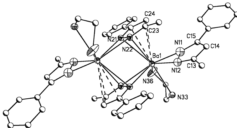
Figure 6. Molecular representation of [{\text{Ba}}(\text{MePhpz})_2(\text{tmeda})]_2 ( 5 ). Disordered components have been removed for clarity.
