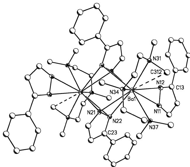
Figure 3. [{\text{Ba}}(\text{Phpz})_2(\text{pmdta})]_2 ( 2 ) with anisotropic displacement parameters depicting 50% probability. Hydrogen atoms have been removed for clarity.
