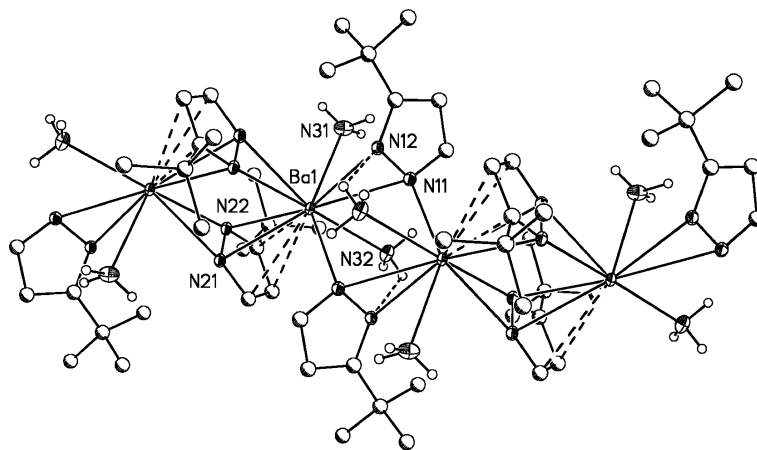
Figure 5. Fragment of [{\text{Ba}}(t\text{Bupz})_2(\text{NH}_3)_2]_n ( 4 ) with anisotropic displacement parameters depicting 50% probability. Hydrogen atoms have been removed from pyrazolate ligands for clarity.
