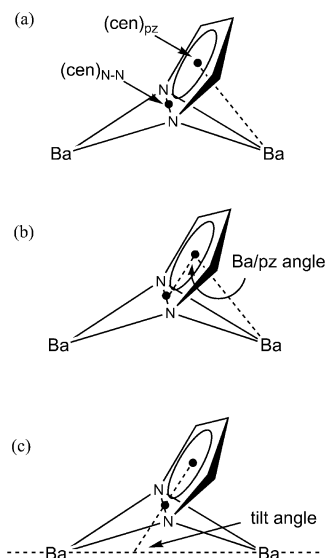
Figure 9. Angles used in structural analysis (a) location of centroids, (b) Ba–cen/pz angle (c) tilt angle.
