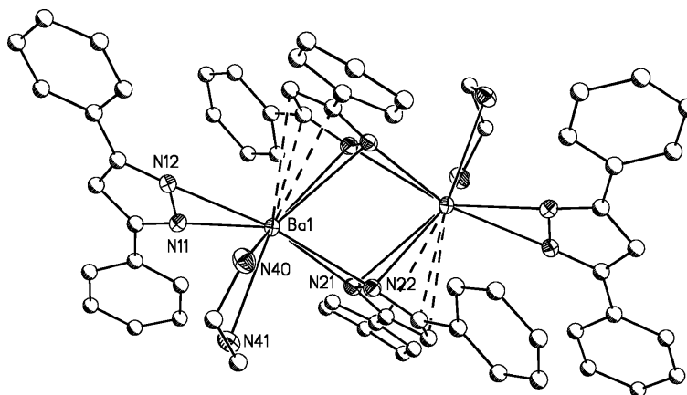
Figure 7. [\{\text{Ba}(\text{Ph}_2\text{pz})_2(\text{tmeda})\}_2]\cdot\text{TMEDA} ( 6 ) with anisotropic displacement parameters depicting 50% probability. The solvent of crystallization TMEDA, hydrogen atoms and TMEDA methyl groups have been removed for clarity.
