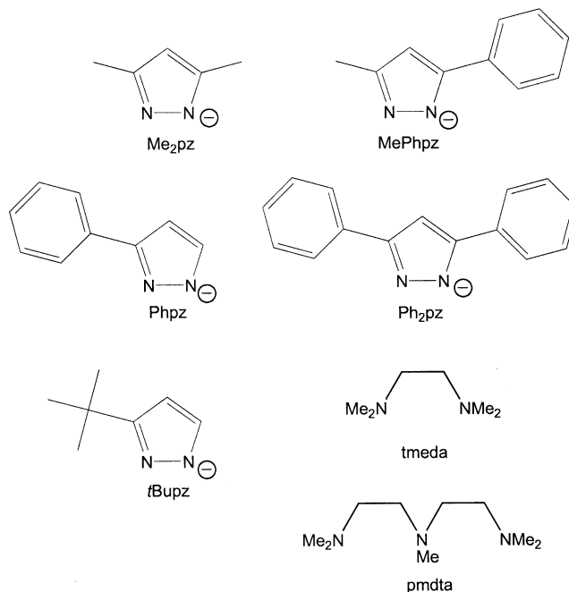
Figure 1. Pyrazolate substitution patterns and neutral donors with abbreviations.
